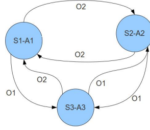
Fig. 2. An Example Finite State Controller
