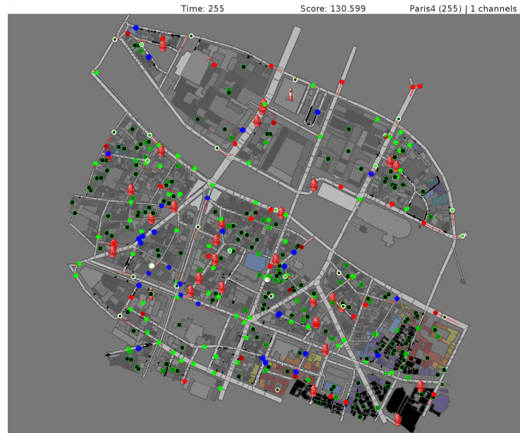
Fig. 4. The final state of Paris4 scenario with RoboAKUT agent
