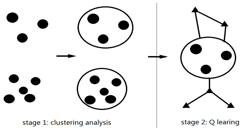
Figure 8. Steps to realize multi-agent coordination
