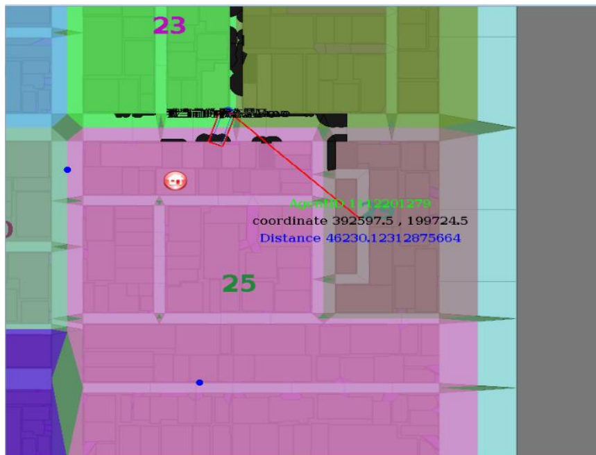
Fig 7.Partition assign
