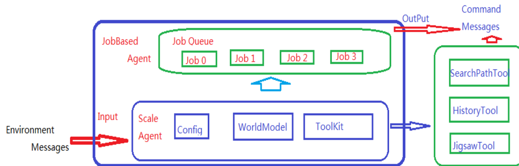
Figure.1 Software Architecture
