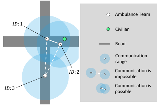
Fig. 2: Example of agents and tasks
