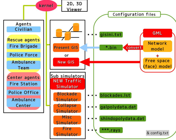
Fig. 2. System architecture including our traffic environment. (Our new traffic simulator works for both the present GIS and the new GIS.)
