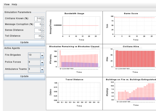
Fig. 2. ECSKernel Control Panel.
