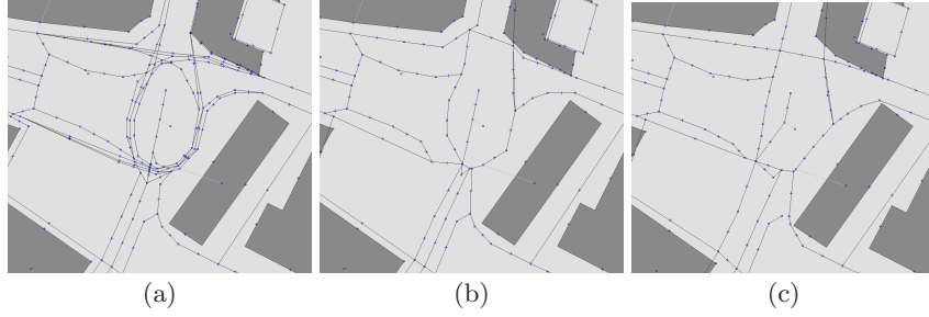
Fig. 2. This figure shows the steps of our road simplification algorithm. (a) a complex junction with multiple lanes (b) the same junction after lane merging (c) the final result after smoothing.
