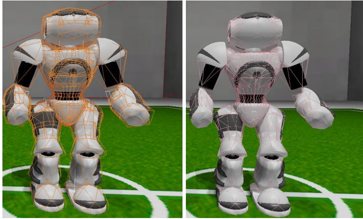
Fig. 4: The left picture shows the PhysX collision model, the right picture the Unreal Engine collision model.
