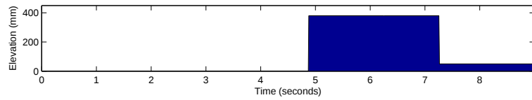
Fig. 9: Elevation \delta below the AR.Drone over time. The elevation increases to approximately 40cm when flying above an obstacle. The elevation is decreased when the obstacle is out of the ultrasound sensor's range. There is a small error between both elevation events, resulting in a small false elevation ( \pm 50mm ) after the AR.Drone flew over the obstacle and is flying above the floor again.
