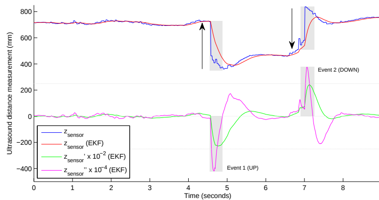
Fig. 8: Response of the ultrasound sensor when flying over an object of approximately (60, 60, 40)\text{mm} . The light-gray lines indicate the threshold \gamma_{\text{elevationEvent}} and null-line. When the second order derivative (magenta line) exceeds the threshold, an event is started (lightgrey rectangle). An event ends when the derivative swaps sign. Each arrow indicates the change in elevation caused by the event. The first event increases the elevation when entering an object and the second event decreases the elevation when leaving the object. Between both events, the AR.Drone performs an altitude correction, as can be seen by the relatively slow increase of distance. This increase is not informative about the elevation and is ignored by the elevation mapping method.
