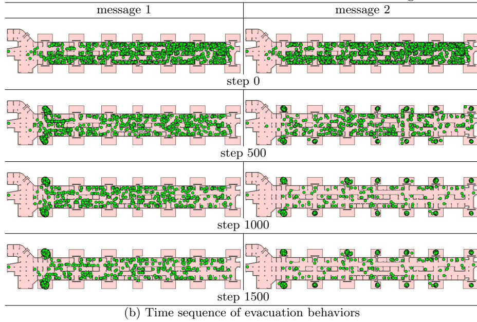
Fig. 3. Simulations of evacuations at subterranean shopping mall
