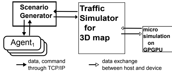
(a) architecture of prototype system
