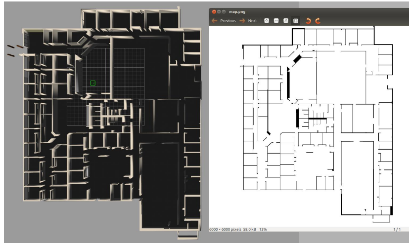
Fig. 2. Screenshot of 3D environment(left) and it's ground truth information(right). Ground truth information is used to calculate received Wi-Fi radio wave power strength between Wi-Fi base station and a robot or between multiple robots
