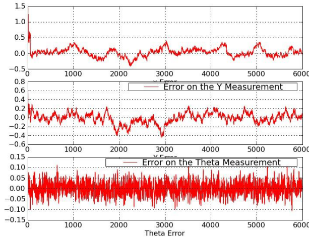
Fig. 7. Error of SLAM algorithm with steps evolution: a) error in X axis (in meters); b) error in Y axis (in meters); c) error in angle (in radians).
