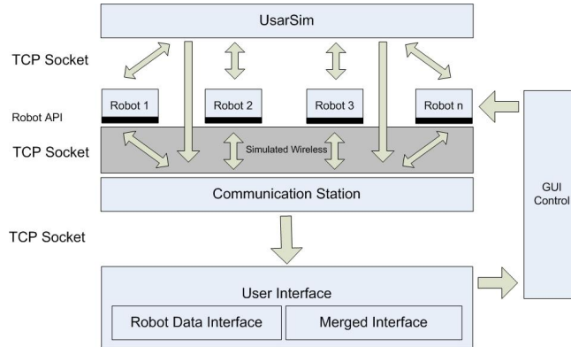
Fig. 1. Brasil-VR Controller Architecture
