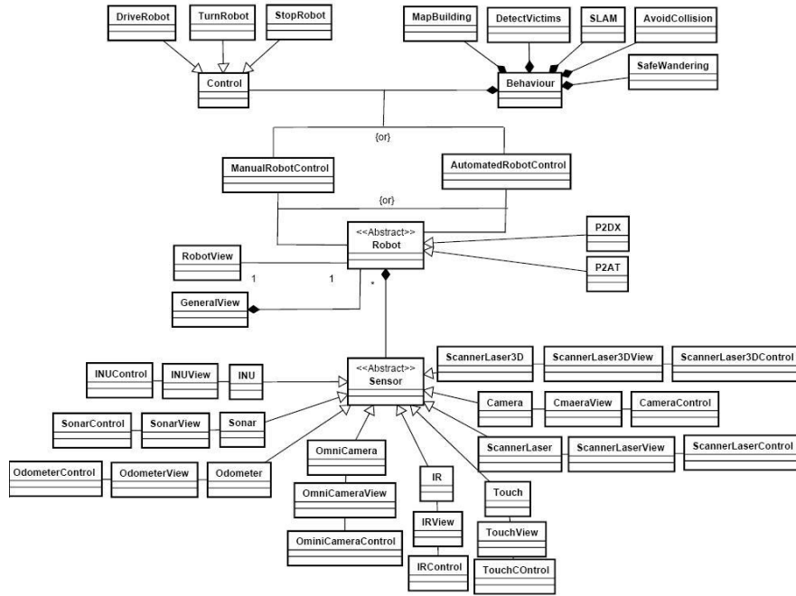
Fig. 2. Brasil-VR Controller Basic Class Diagram
