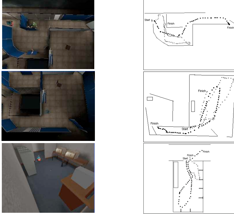
Fig. 6. Results. Left: Indoor scenes with real-world-like obstacles. P2DX shown pose is the initial robot pose in each test. Right: evolution of robot path. Filled points represent robot path with the neurofuzzy controller, while empty points show robot path with pure behavior-based controller.
