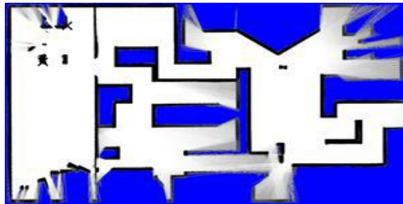
Fig. 1. A Generated map using GSLAM and Grid Mapping
