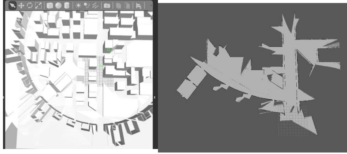
(a) Layout with displays in the model of Hall 1 (b) Output of hector_SLAM
