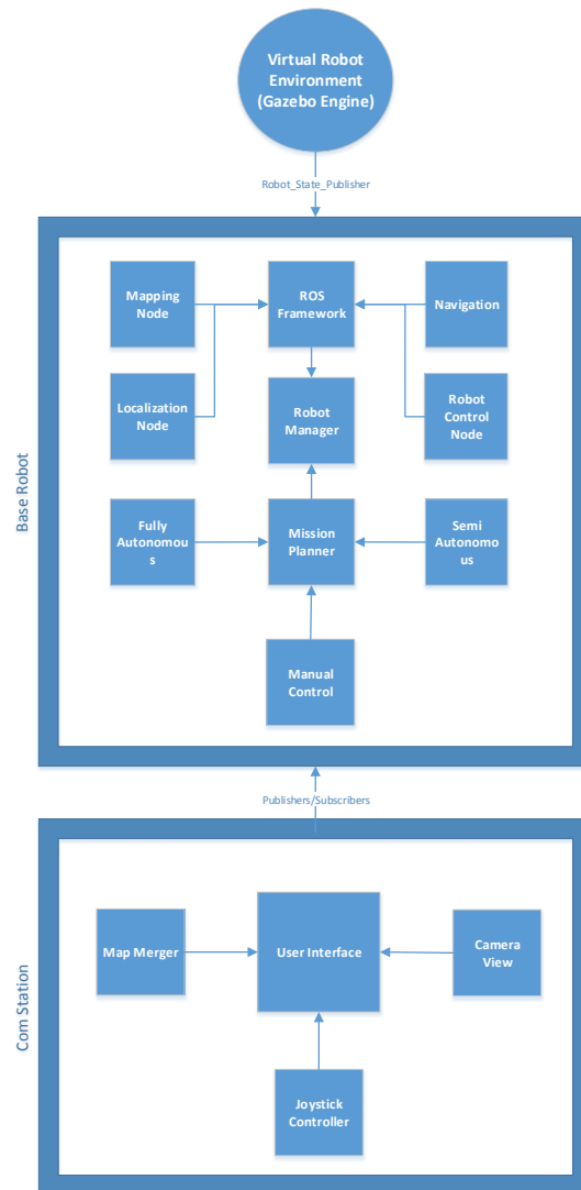
Fig 1: System Architecture
