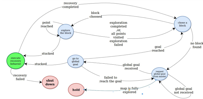
Fig. 1. The state machine of robot during exploration, Red color indicates a final outcome, Blue indicates a state, and Green indicates another state machine.
