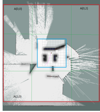
Fig. 2. The red square is the global costmap and the blue square is the local costmap. note that A(0,2) is fully unknown while A(2,0) is almost fully explored.
