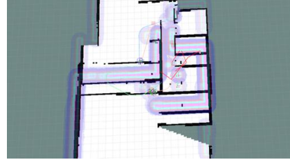
Fig. 4: rrt_exploration with 3 robots autonomously exploring the world
