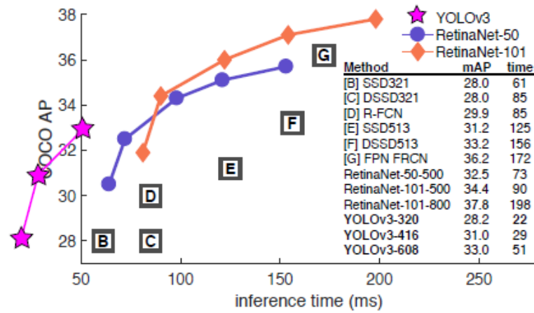
Figure 2: Yolov3 is faster than others [11]
