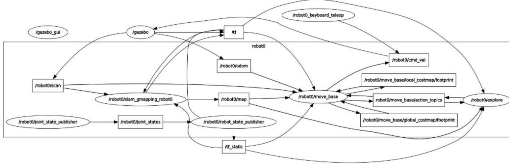
Fig 3. Robot node with its SLAM, Navigation and Exploration stacks
