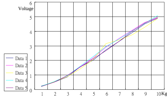
Fig. 5. The measured signals of one strain gauge in five tries.
