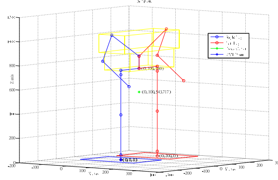
Fig. 1. The kinematic design of a humanoid robot.
