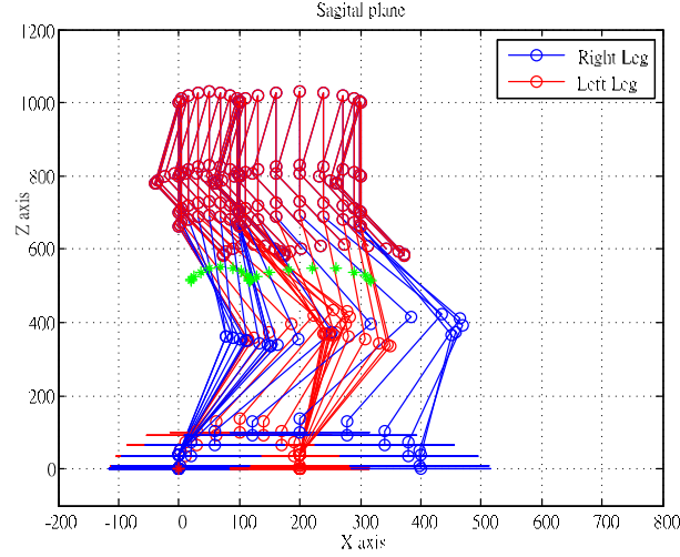
Fig. 2. The stick diagram of the humanoid robot for a walking step.
