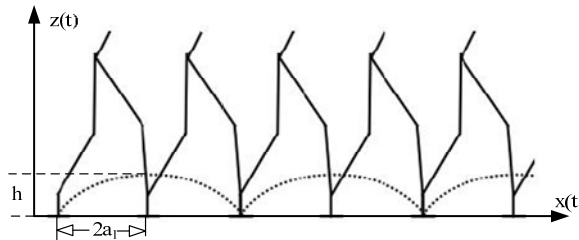
Fig. 7. The cycloid used for the humanoid walking pattern.
