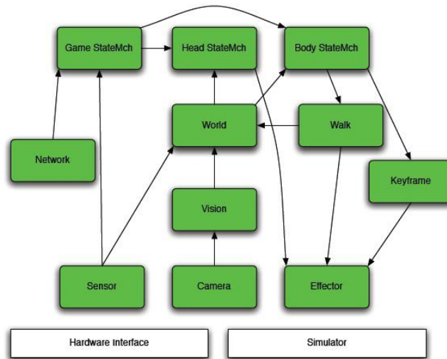
Fig. 3. Software architecture
