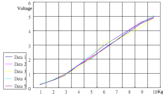
Fig. 5. The measured signals of one strain gauge in five tries.
