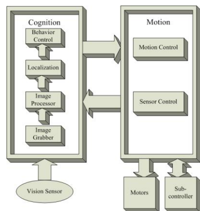
Fig. 3-1. Software Architecture
