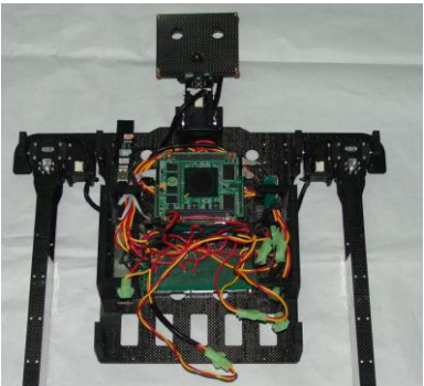
Fig.2-4. The control system of THU_Strider
