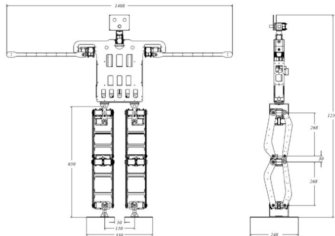
Fig. 2-2. Dimensions of THU_Strider
