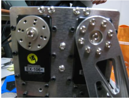
Fig. 2. The joint of humanoid robot.
