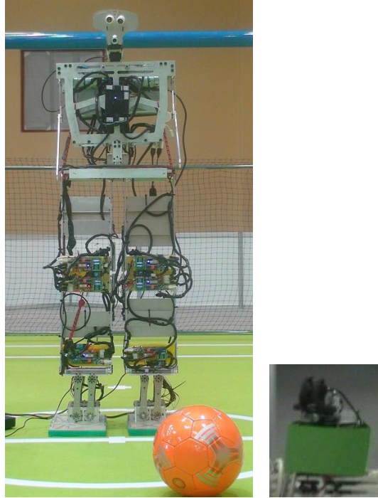
Fig. 4. Photos of assembled HuroEvolution AD (left-hand-side) and the active vision sensor (right-hand-side)
