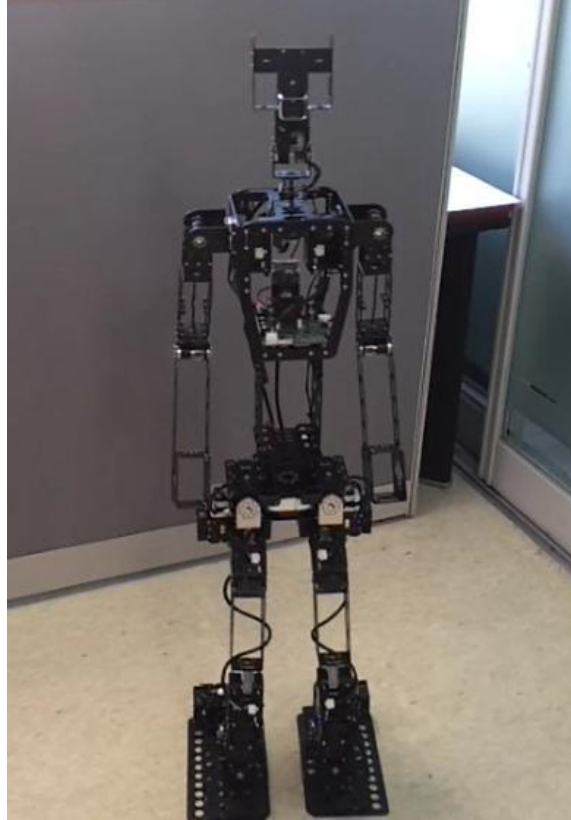
Figure.1 Unfinished Robot
