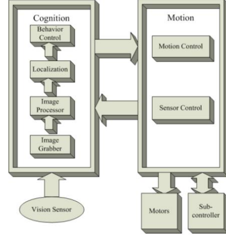
Fig. 4. Software Architecture
