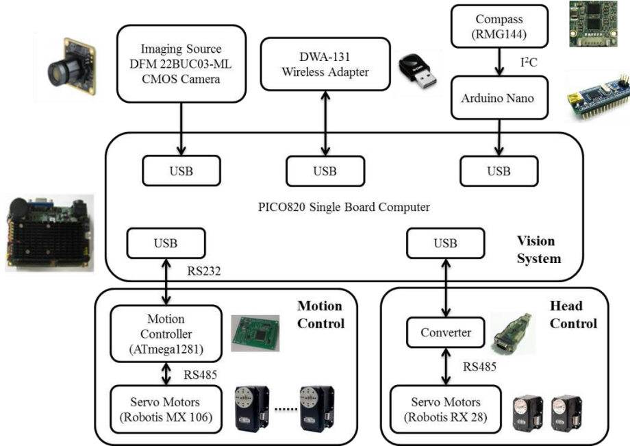
Fig. 3. Control architecture of HuroEvolution robot.
