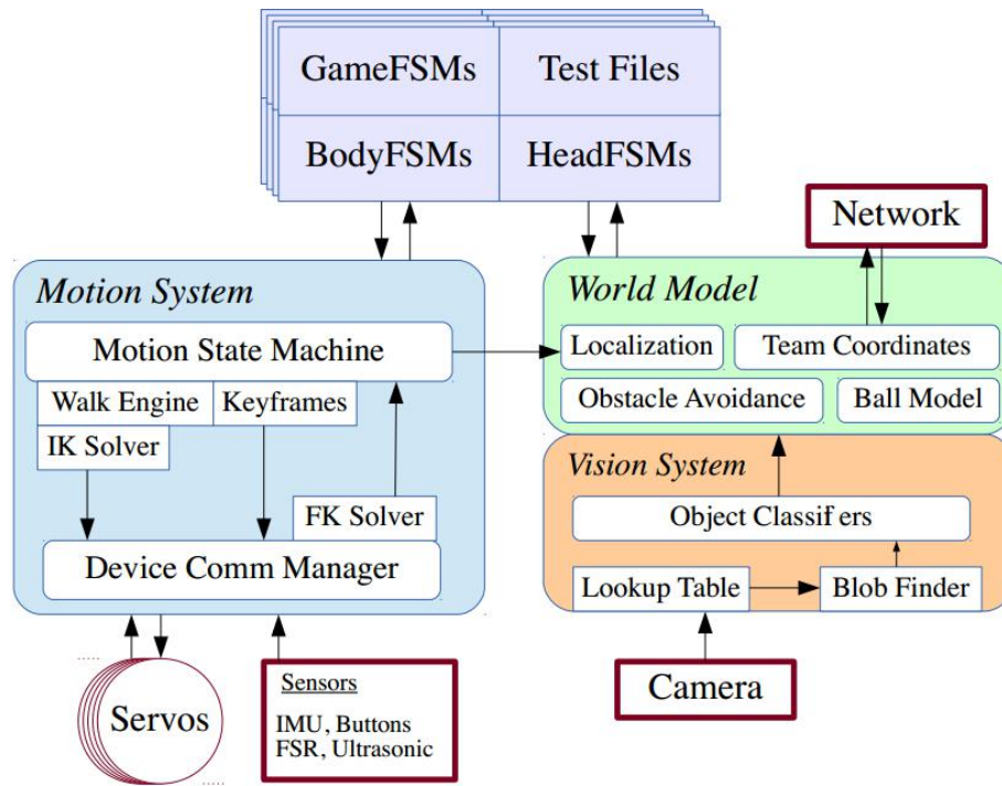
Fig 5: Software Architecture
