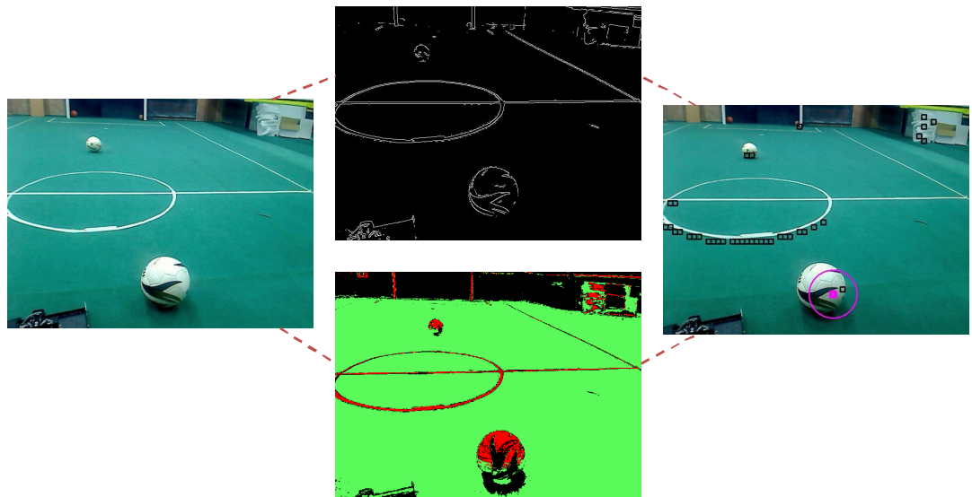
Fig. 8. Ball Detection Steps
