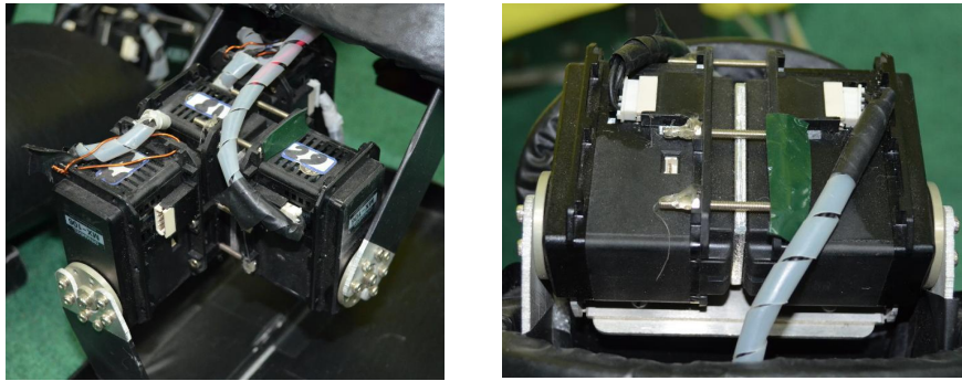
Fig. 4. Dual motor used as an actuator (Left is Ankle, Right is Knee)
