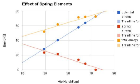
Fig.5. Effect of Spring Elements
