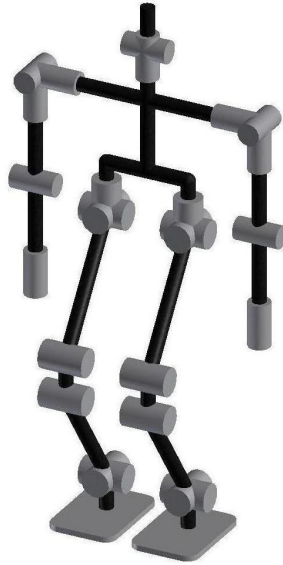
Fig. 2. Degree-of-freedoms configuration of the new RESr
