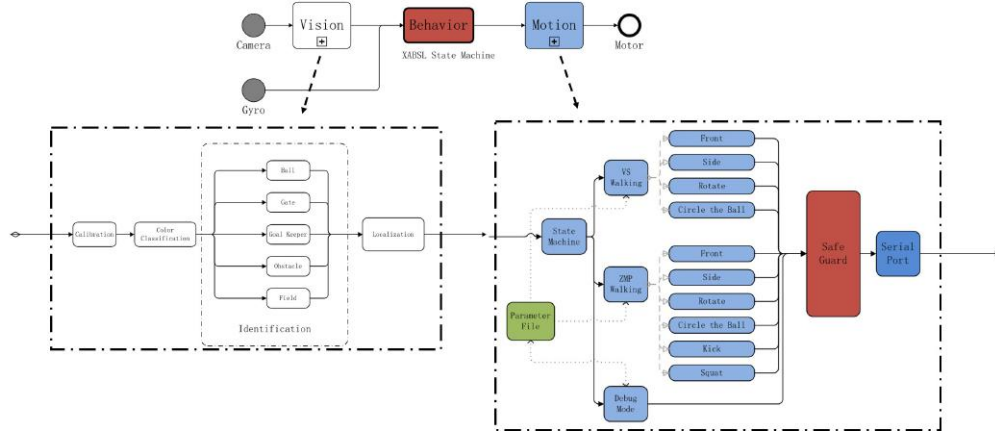
Fig. 3. Software Architecture
