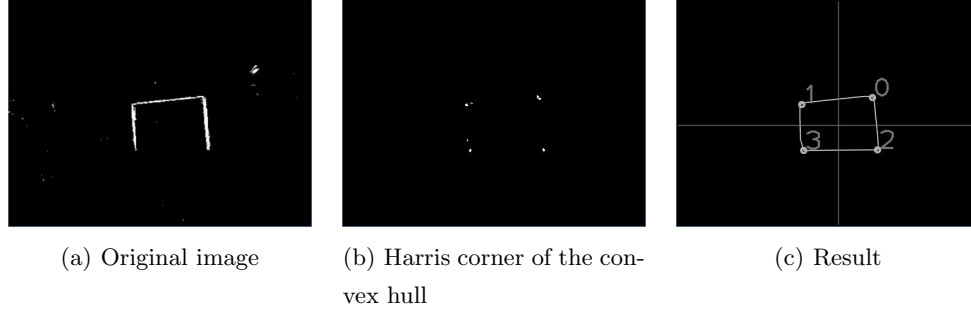
Fig. 5. Goal detector
