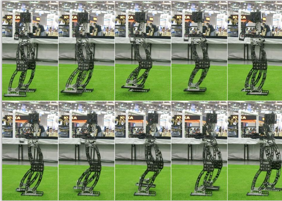
Fig. 3. Enhanced generated trajectory of Baset Adult-Size robot
