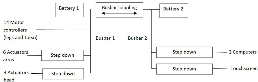
Fig. 4. Sweaty II's power supply
