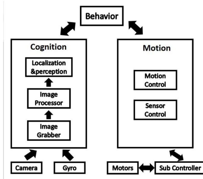
Fig. 3. Software Architecture
