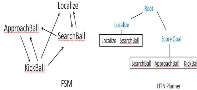
Fig.3. Comparison between two AI architectures
