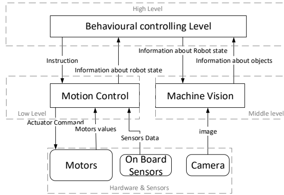
Fig. 3. Diagram of IRC humanoid robot software architecture
