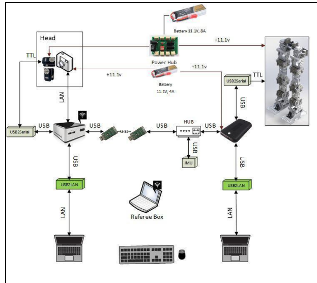
Fig. 2. Electronical design of Artin robot
