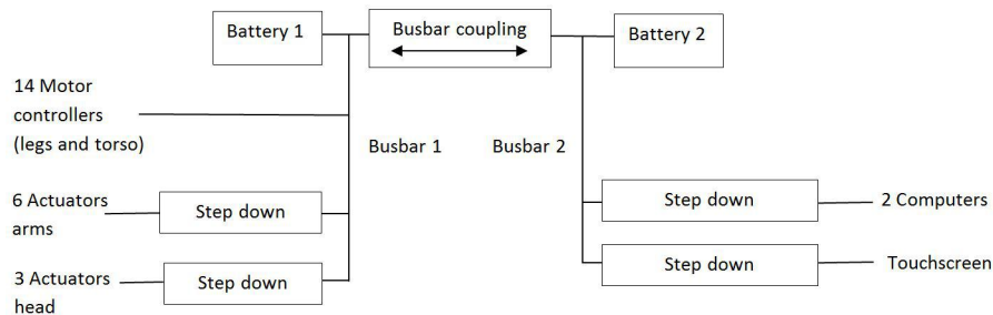
Fig. 5. Sweaty II's power supply.
