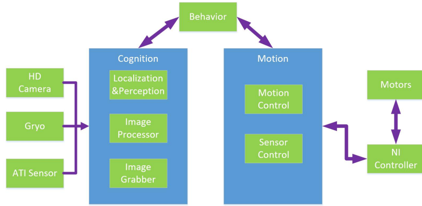
Fig. 3. Software Architecture
