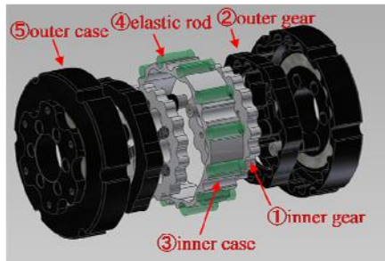
(a) structure of the mechanism
