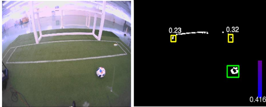
Fig.5 Distinguishing ball and goalpost
