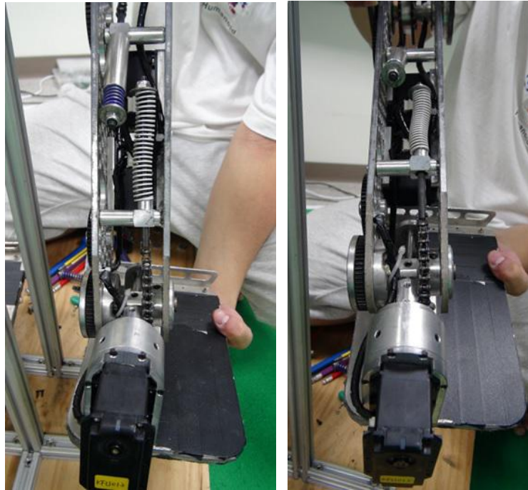
Fig. 2. The detail photo of NKFUST humanoid ankle. As shown in the photo, the extra gear and spring are design for the ankle join to have stronger torque.
