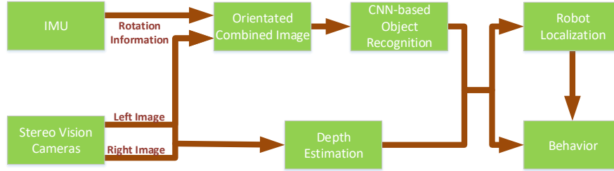
Fig. 4. Visual Perception System Overview
