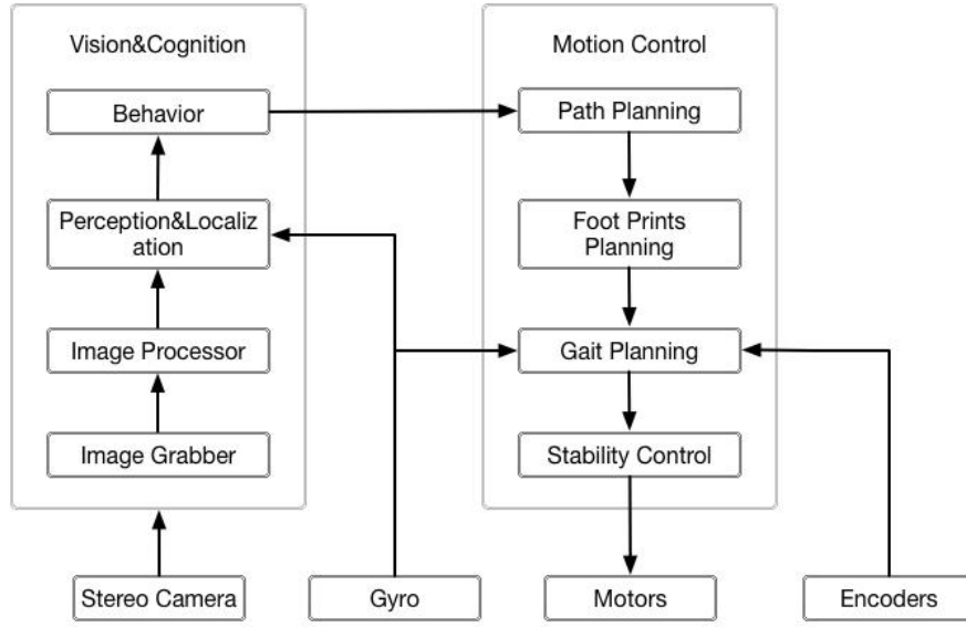
Fig. 3. Software Architecture
