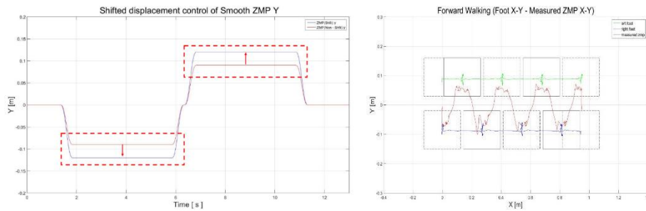
Fig. 4. The modified ZMP reference curve (left) and the measured ZMP movement (right)
