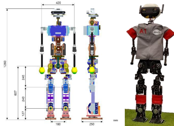
Fig. 2. 3D CAD design of ALICE (left), Actual appearance (right)
