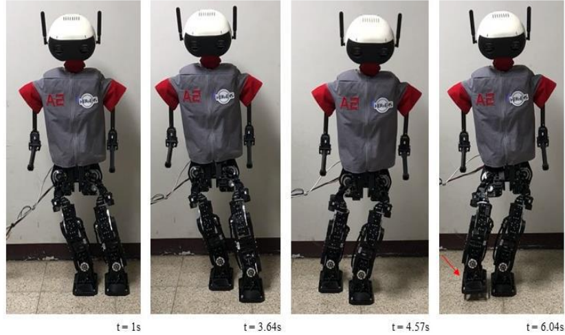
Fig. 5. Walking Experiment with the shifted displacement ZMP walking method (forward walking)
