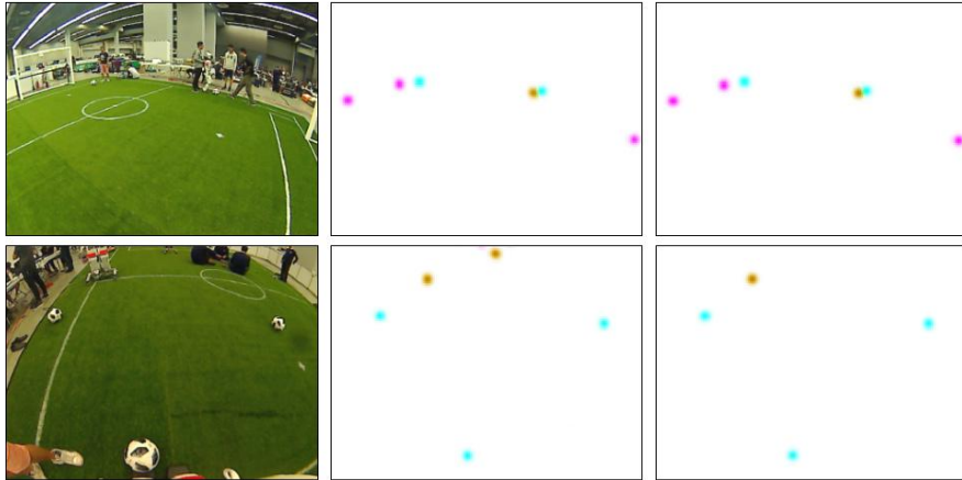
Fig. 4. Left column: A captured image from the robot in the test set. Middle column: The output of the network with balls (cyan), goal posts (magenta), and robots (yellow) annotated. Right column: Ground truth.
