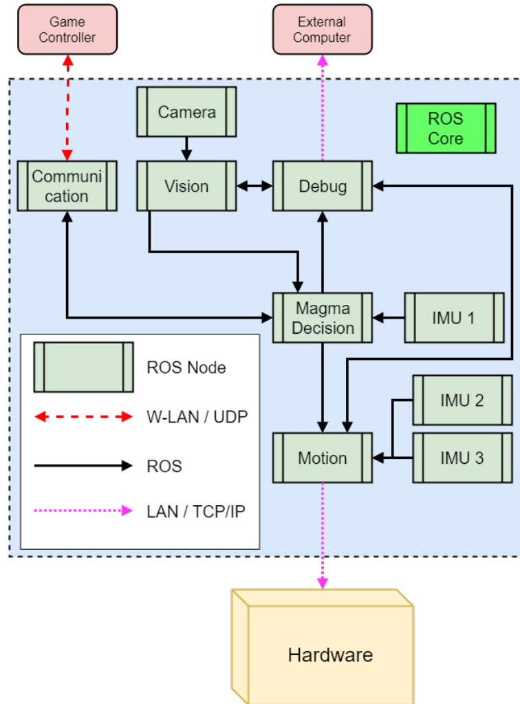
Fig. 2. Sweaty's new software architecture.
