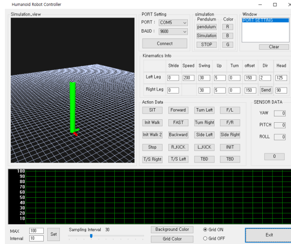
Fig. 3. motion software
