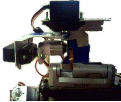
Fig. 1. The Pan and Tilt Unit of Abarenbou. The servos are mounted upside down to prevent stress on the thin ribbon cable.
