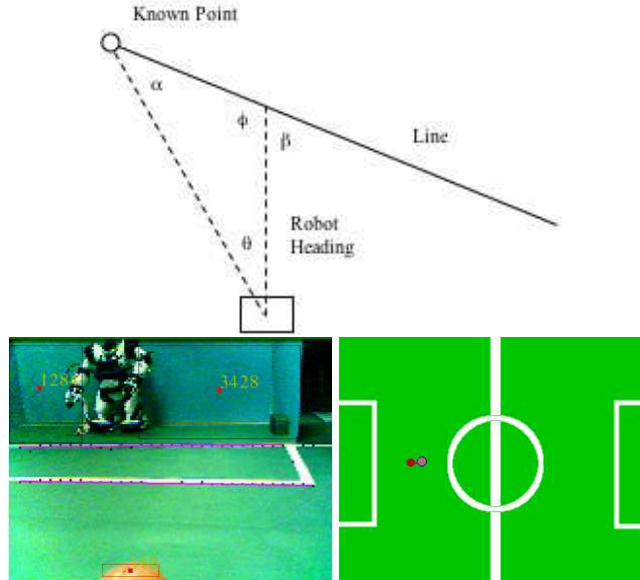
Fig. 5. Localizing using a known point, its relative position, and relative orientation of a line. Image from the robot with highlighted line segments and the calculated position are shown in the lower image.
