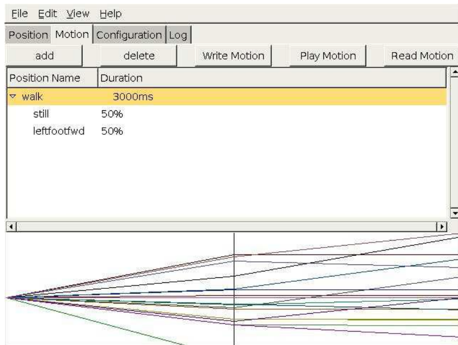
Fig. 4. Interface of our motion development system. The top window shows the development of a position, the bottom window shows the combination of these positions into motions.
