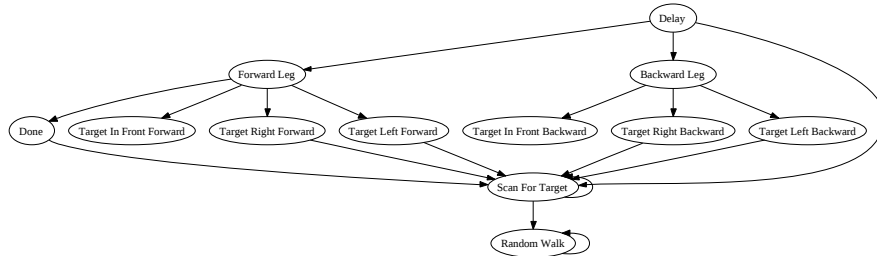
Fig. 6. Automatically generated state transition graph for a simple approach and avoid task. Solid lines are state transitions.
