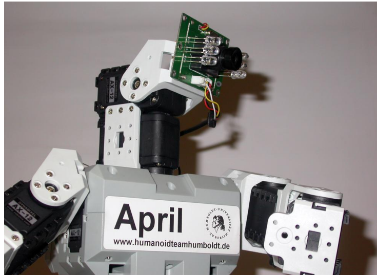
Fig. 2. Pan-and-tilt camera module.
