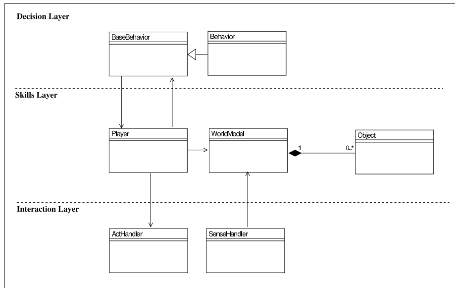
Fig. 3. UML class diagram of the Object Oriented Framework
