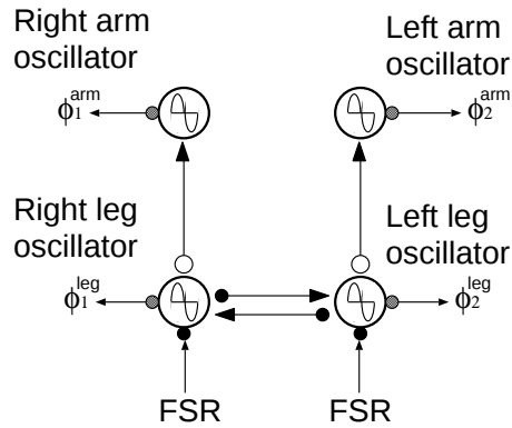
Fig. 9. A phase control system
