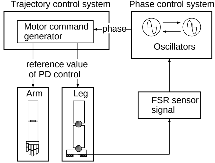
Fig. 8. A walking control system
