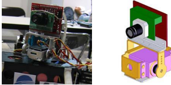
Fig. 8. Pan-tilt mechanism used on-board the humanoid robot
