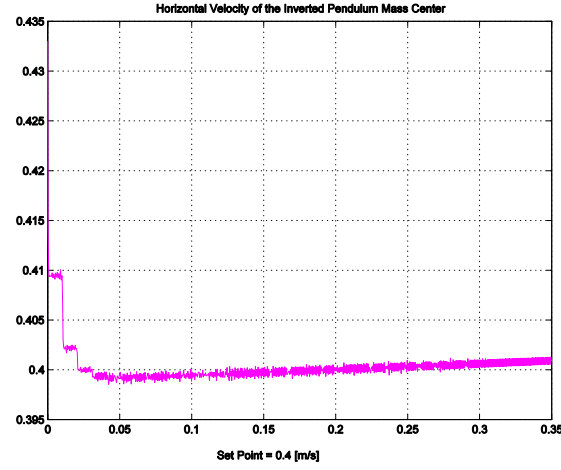
Fig. 5. Horizontal velocity of the CM is regulated at 0.4[m/s]
